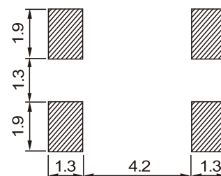
SOLDER PATTERN
