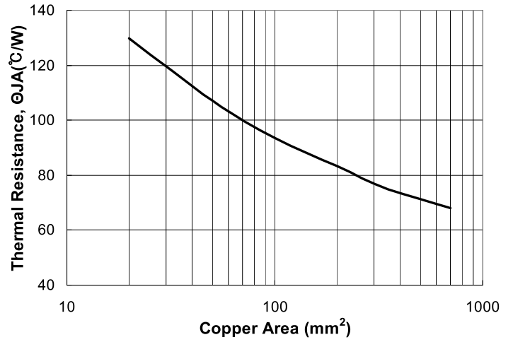
Thermal Resistance( \theta_{JA} ) vs. Copper Area (SOP-8)
