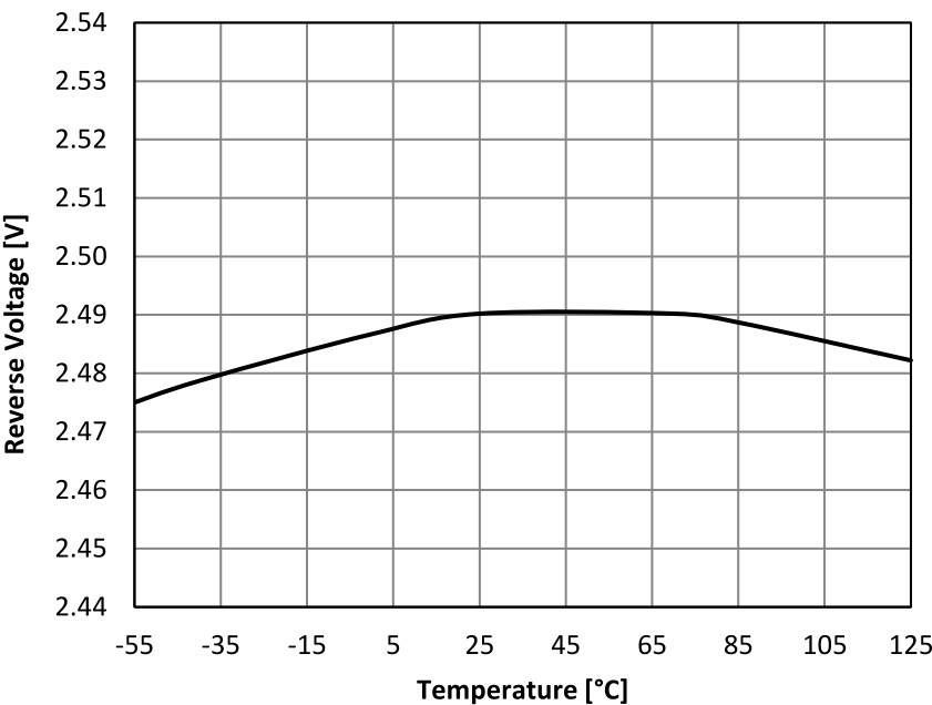
Temperature Drift
