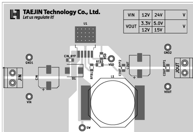
Figure 28. PCB Layout Example
