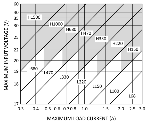
Figure 24. LM2576-15
