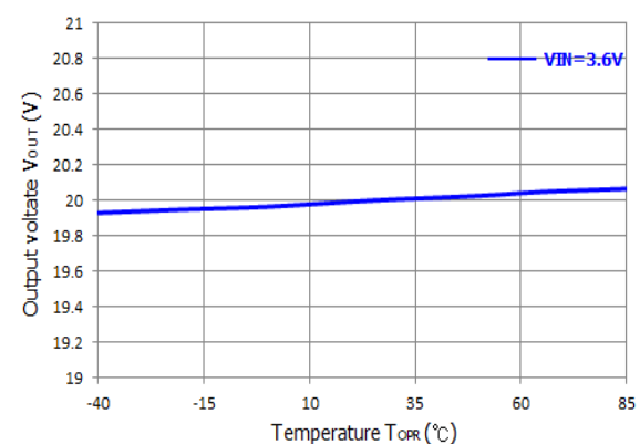
Output voltage vs Temperature ( V_{OUT}=20V )
