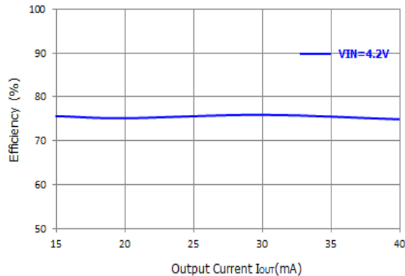
Efficiency vs Output Current ( V_{OUT}=20V )
