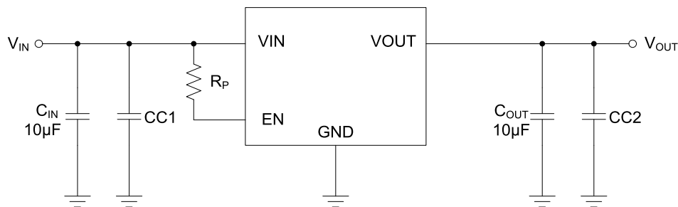
Fig. 1. Application with Decoupling Capacitor, CC1 & CC2
