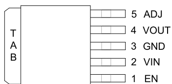
TO-252-5L
