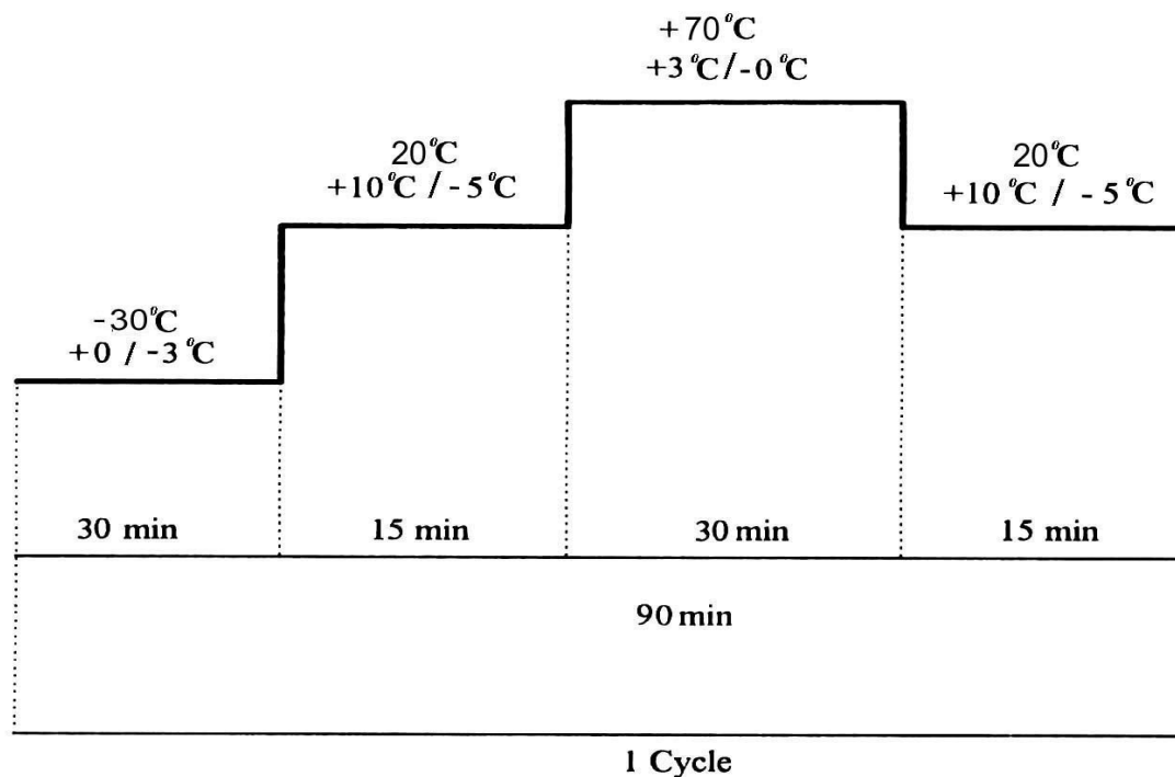
Fig.3 Temp. Cycle test:
