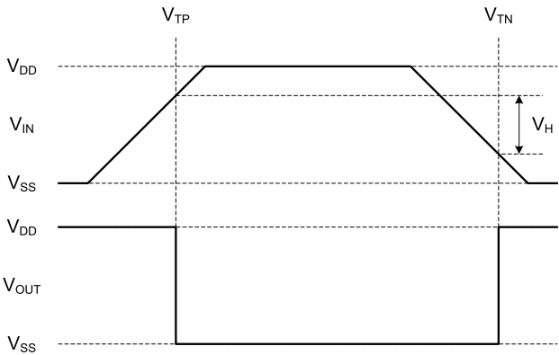
Fig. 1. Hysteresis Definition
