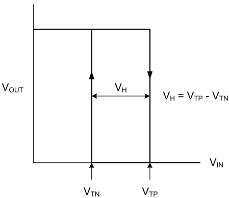
Fig. 2. Hysteresis Characteristic
